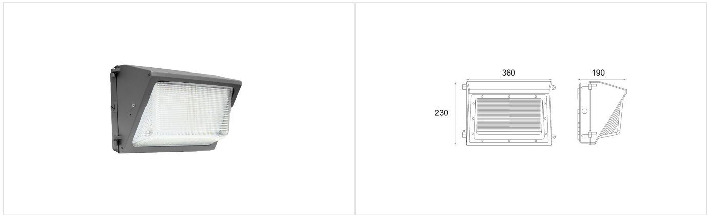
Wallpack light
